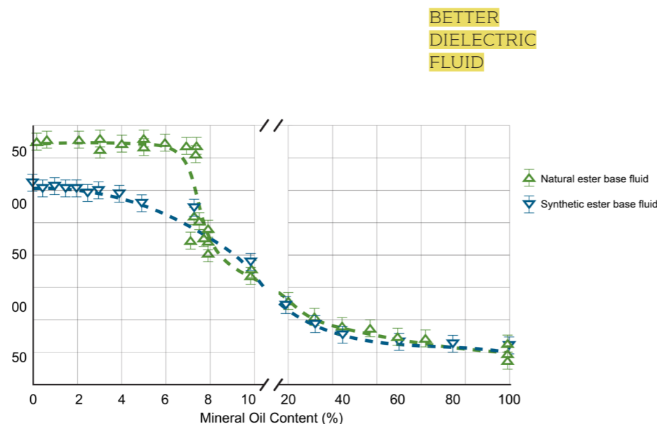
Figure 1. Fire points of natural and synthetic ester fluids at different residual mineral oil contents
