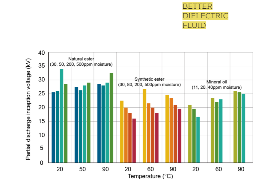
Figure 2. Partial discharge inception voltage of natural ester, synthetic ester and mineral oil as measured according to IEC TR 61294:1993 at different temperatures and moisture levels
