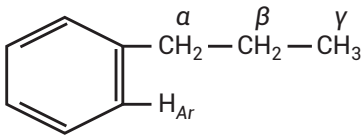
Figure 1. Hydrogen types in a molecule
