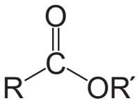
Figure 2. Structure of an ester
