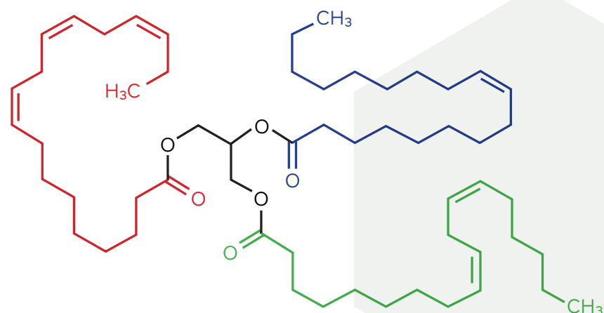
Figure 3. Structure of natural ester
