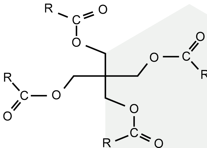
Figure 4. Structure of synthetic ester
