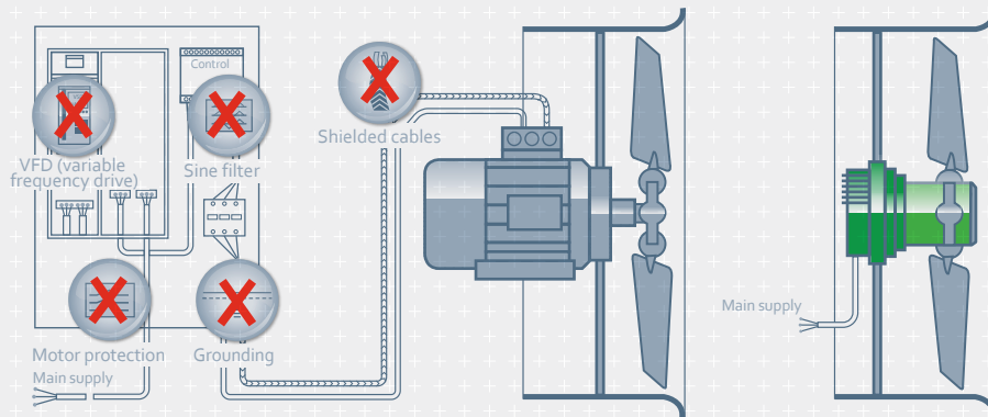
Figure 5. EC technology with unsurpassed compactness
