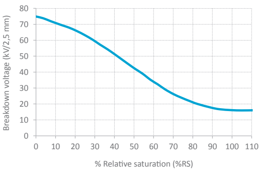
Figure 1. Dependency between breakdown voltage and water content in the insulating liquid [1]
