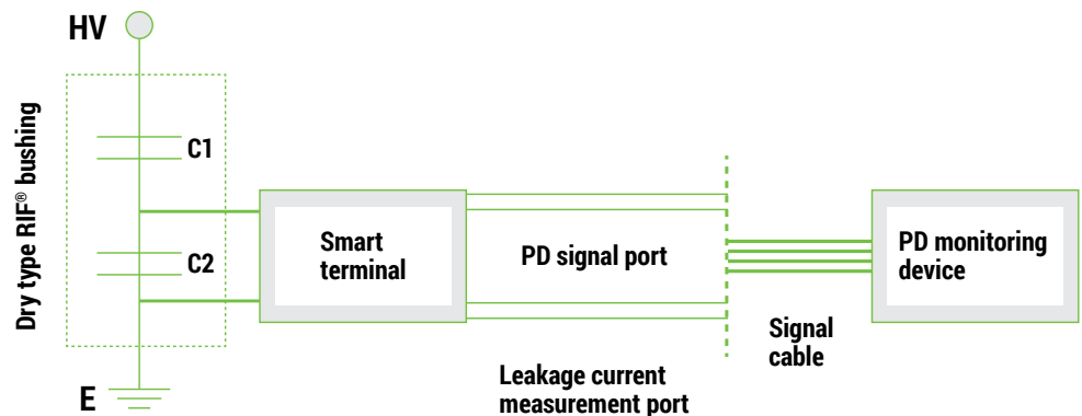
Figure 2. Signal coupling
