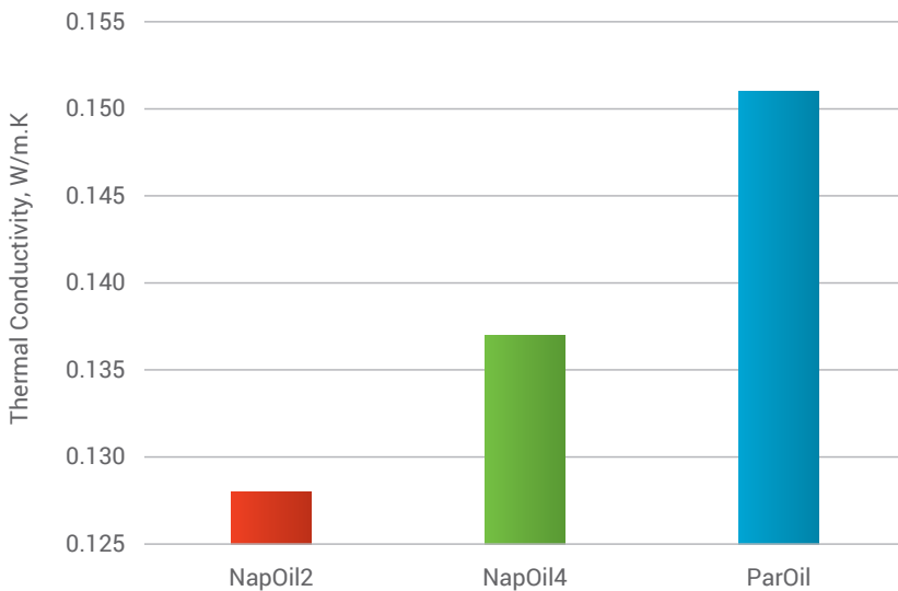
Figure 8. Thermal conductivity at 80°C by PLTL-73
