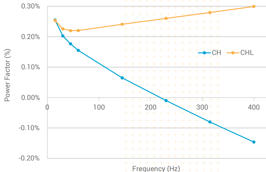
Figure 2. Variable Frequency Power Factor results for a Kuhlman 118 kV transformer
